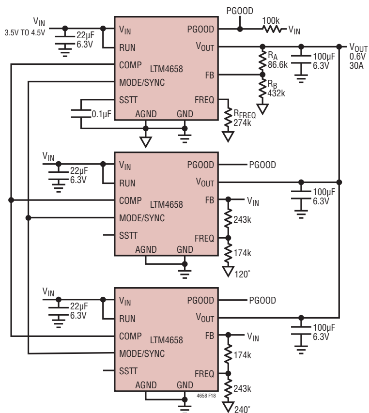
Figure 18. Three-Phase Application
