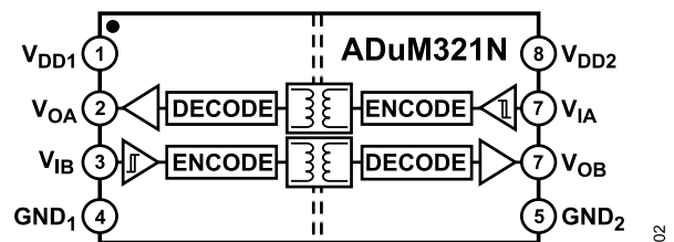
Figure 2. ADuM321N Functional Block Diagram
