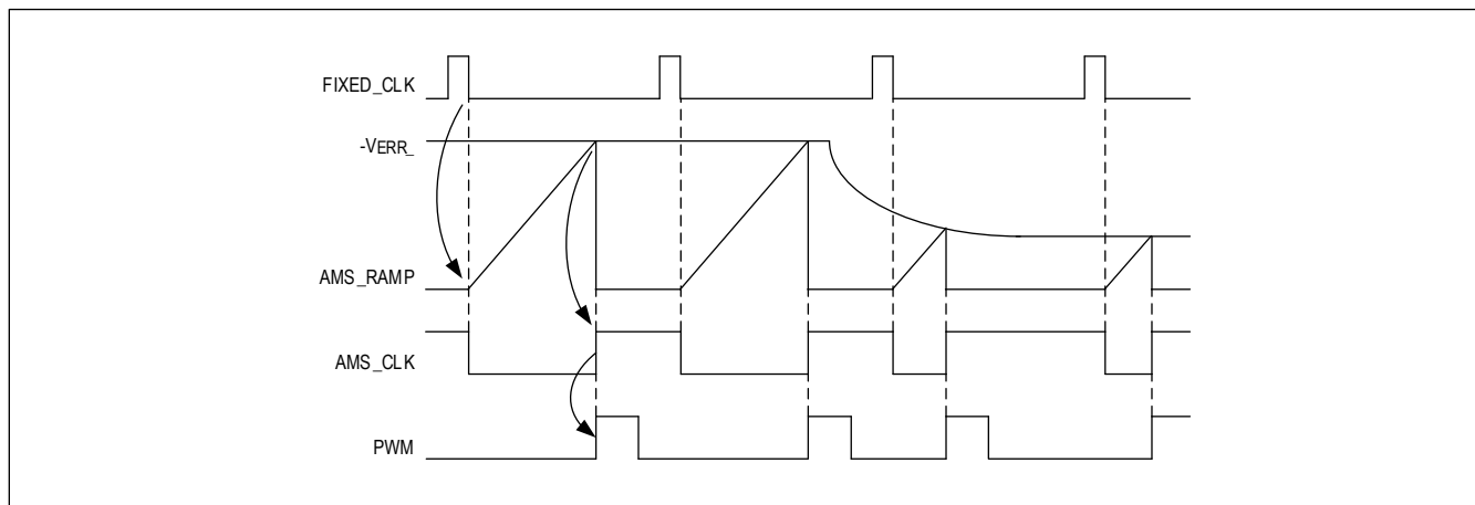
Figure 2. AMS Operation
