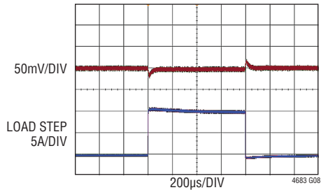
Single Channel Load Transient Response (0A) to (10A) Load Step, 10A/ \mu\text{s} , V_{\text{IN}} = 12\text{V} , V_{\text{OUT}} = 0.7\text{V} , f_{\text{SW}} = 575\text{kHz}
