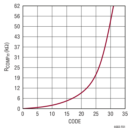
Figure 1. Programmable R_{COMPn}
