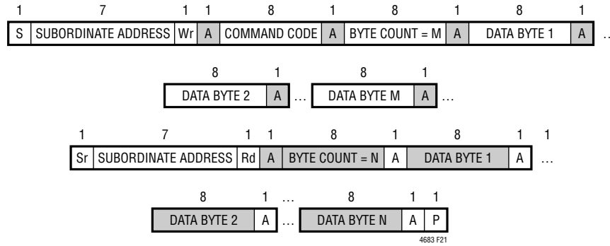
Figure 21. Block Write – Block Read Process Call
