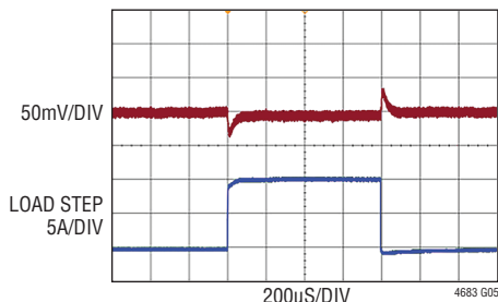
Single Channel Load Transient Response (0A) to (10A) Load Step, 10A/ \mu\text{s} , V_{\text{IN}} = 12\text{V} , V_{\text{OUT}} = 0.3\text{V} , f_{\text{SW}} = 250\text{kHz}
