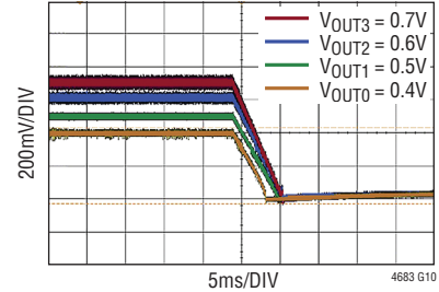
FIGURE 48 CIRCUIT, 12V_{IN} , 10A ON V_{OUT0} NO LOAD ON OTHER OUTPUTS AND 180mV PRE-BIAS ON V_{OUT0}
