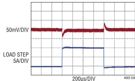
Single Channel Load Transient Response (0A) to (10A) Load Step, 10A/ \mu\text{s} , V_{\text{IN}} = 12\text{V} , V_{\text{OUT}} = 0.4\text{V} , f_{\text{SW}} = 350\text{kHz}
