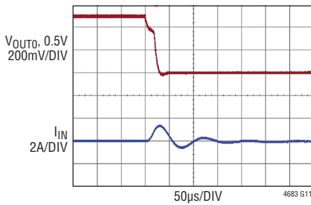
FIGURE 48 CIRCUIT, 12V_{IN} , NO LOAD ON V_{OUT0} PRIOR TO APPLICATION OF SHORT-CIRCUIT USE HIGH RANGE OF I_{OUT} SYSTEM SHORT-CIRCUIT USING LOW IMPEDANCE COPPER ACROSS OUTPUT (HARD SHORT)
