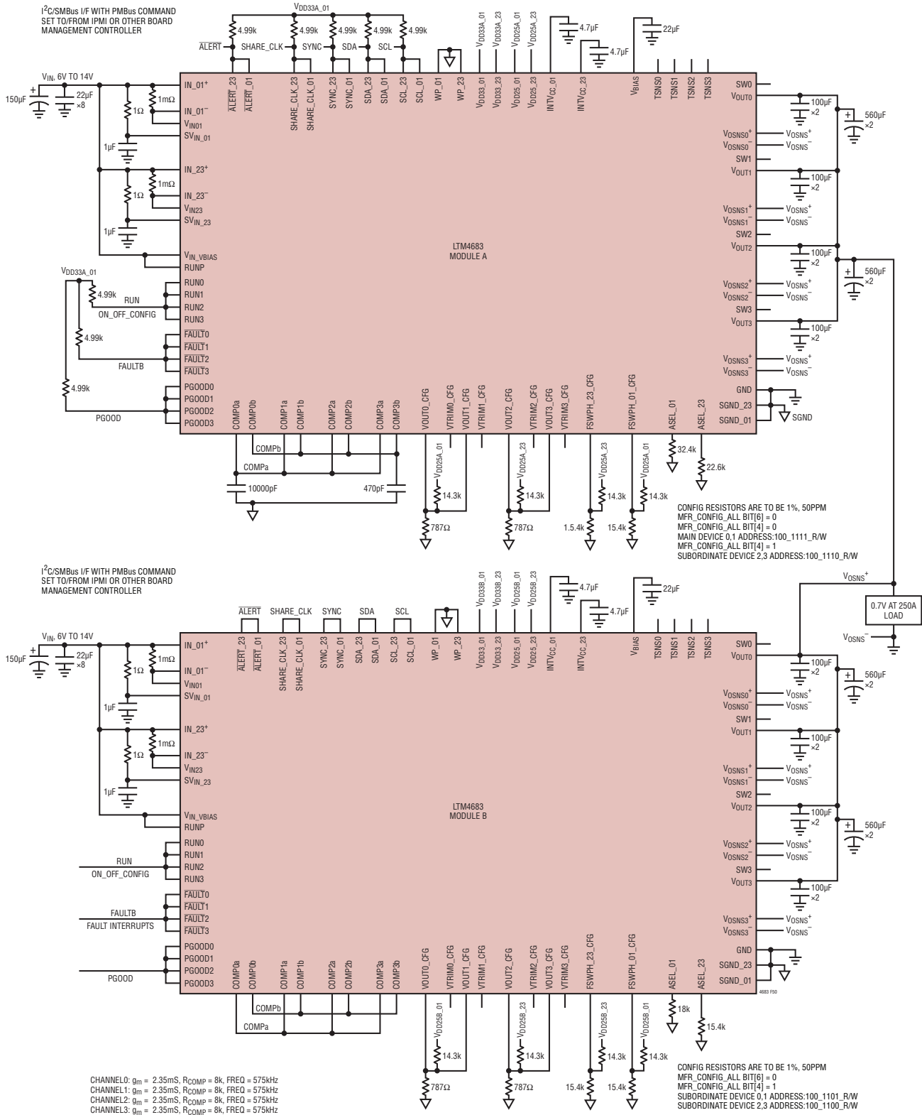
Figure 50. Two Paralleled LTM4683 Producing 0.7V OUT at 250A. Integrated Power System Management Features Accessible Over 2-Wire I 2 C/SMBus/PMBus Serial Interface
