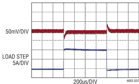
Single Channel Load Transient Response (0A) to (10A) Load Step, 10A/ \mu\text{s} , V_{\text{IN}} = 12\text{V} , V_{\text{OUT}} = 0.6\text{V} , f_{\text{SW}} = 500\text{kHz}
