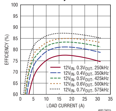
Channel Efficiency vs Load Current
