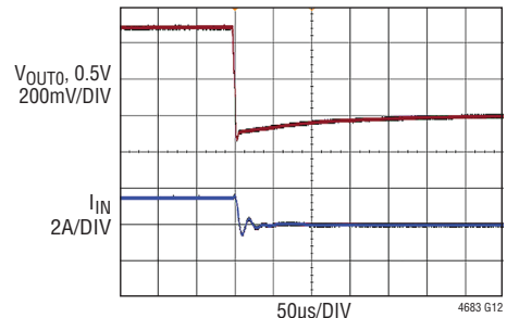
FIGURE 48 CIRCUIT, 12V_{IN} , 31.25A LOAD ON V_{OUT0} PRIOR TO APPLICATION OF SHORT-CIRCUIT USE HIGH RANGE OF I_{OUT} SYSTEM SHORT-CIRCUIT USING LOW IMPEDANCE COPPER ACROSS OUTPUT (HARD SHORT)
