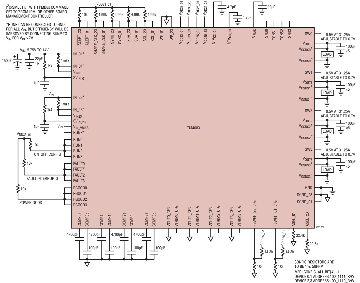
Test Circuit 1.
