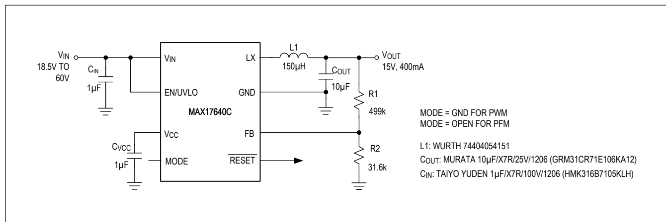
Figure 10. 15V, 400mA Step-Down Regulator
