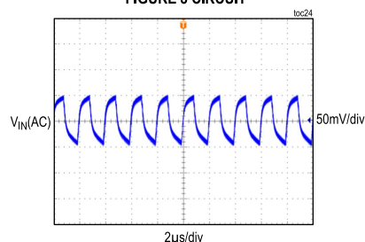
MAX17640C INPUT VOLTAGE RIPPLE FIGURE 8 CIRCUIT
