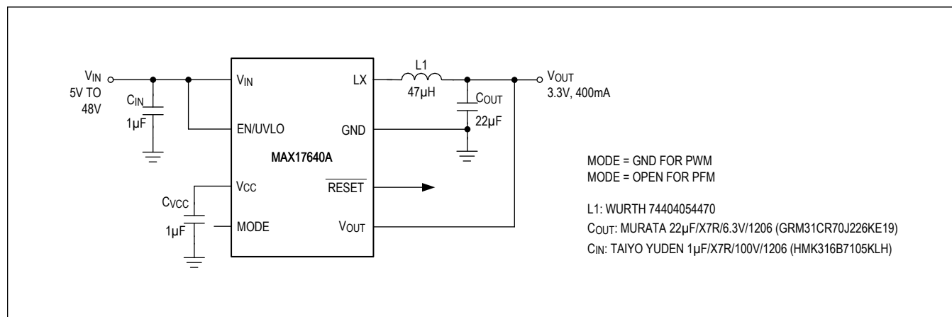
Figure 5. 3.3V, 400mA Step-Down Regulator
