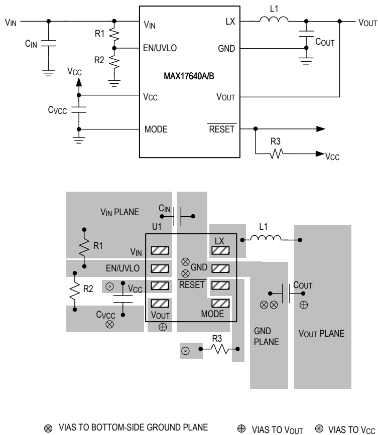
Figure 3. Layout Guidelines for MAX17640A and MAX17640B
