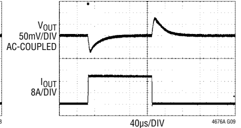
FIGURE 35 CIRCUIT AT 5\text{V}_{\text{IN}} . \text{VOUT\_COMMAND}_n SET TO 1.000\text{V} . 0\text{A} TO 20\text{A} LOAD STEP AT 20\text{A}/\mu\text{s}
