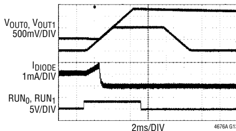
FIGURE 69 CIRCUIT AT 12\text{V}_{\text{IN}} . 77\text{m}\Omega LOAD ON \text{V}_{\text{OUT}0} , 500\Omega ON \text{V}_{\text{OUT}1} . \text{V}_{\text{OUT}1} PRE-BIASED THROUGH A DIODE. \text{TON\_RISE}_0 = 3\text{ms} , \text{TON\_RISE}_1 = 5.297\text{ms} , \text{TOFF\_DELAY}_1 = 0\text{ms} , \text{TOFF\_DELAY}_0 = 2.43\text{ms} , \text{TOFF\_FALL}_1 = 5.328\text{ms} , \text{TOFF\_FALL}_0 = 3\text{ms} , \text{ON\_OFF\_CONFIG}_1 = 0\text{x}1\text{F} , \text{ON\_OFF\_CONFIG}_0 = 0\text{x}1\text{E}
