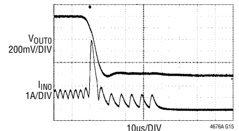
FIGURE 69 CIRCUIT AT 12\text{V}_{\text{IN}} . 77\text{m}\Omega LOAD ON \text{V}_{\text{OUT}0} PRIOR TO APPLICATION OF SHORT CIRCUIT
