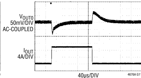
FIGURE 69 CIRCUIT AT 24\text{V}_{\text{IN}} . \text{C}_{\text{OUT}0} = 5 \times 100\mu\text{F} AND \text{V}_{\text{OUT}0} COMMANDED TO 3.300\text{V} . 0\text{A} TO 10\text{A} LOAD STEP AT 10\text{A}/\mu\text{s}
