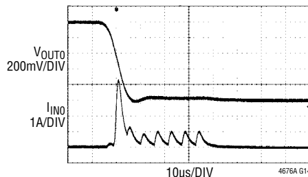
FIGURE 69 CIRCUIT AT 12\text{V}_{\text{IN}} . NO LOAD ON \text{V}_{\text{OUT}0} PRIOR TO APPLICATION OF SHORT CIRCUIT
