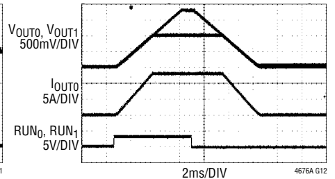
FIGURE 69 CIRCUIT AT 12\text{V}_{\text{IN}} . 77\text{m}\Omega LOAD ON \text{V}_{\text{OUT}0} . NO LOAD ON \text{V}_{\text{OUT}1} . \text{TON\_RISE}_0 = 3\text{ms} , \text{TON\_RISE}_1 = 5.297\text{ms} , \text{TOFF\_DELAY}_1 = 0\text{ms} , \text{TOFF\_DELAY}_0 = 2.43\text{ms} , \text{TOFF\_FALL}_1 = 5.328\text{ms} , \text{TOFF\_FALL}_0 = 3\text{ms} , \text{ON\_OFF\_CONFIG}_n = 0\text{x}1\text{E}
