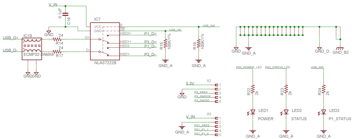
Figure 43: USB Protection
