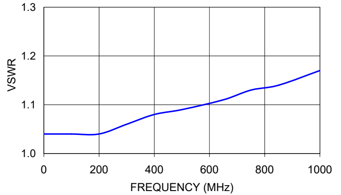
LAT-30+ VSWR
