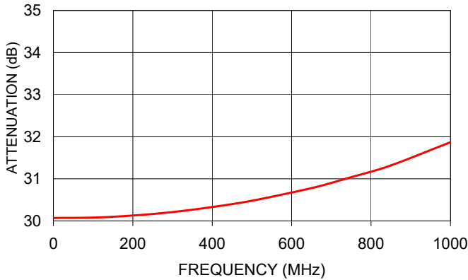
LAT-30+ ATTENUATION
