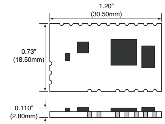
Figure 1: Package Dimensions
