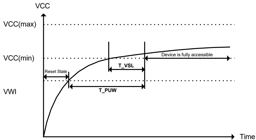
Figure 15-1. Power-On Process
