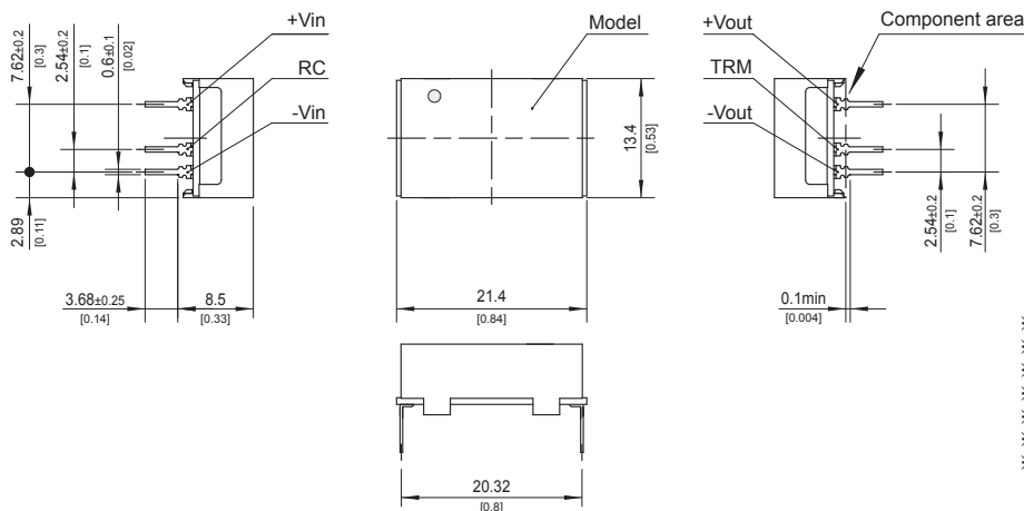
2. DIP(type C)
