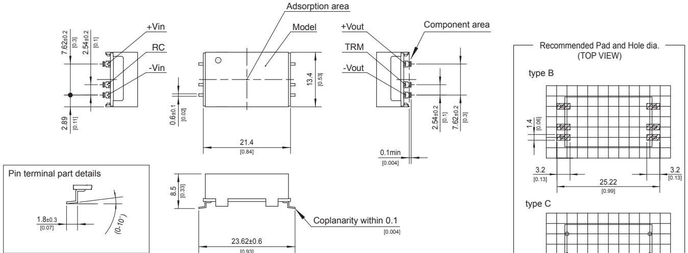
1. SMD(type B)
