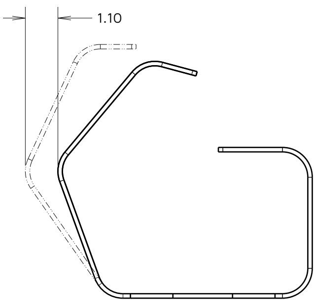
S1991-46R DEFLECTION FROM FRONT
