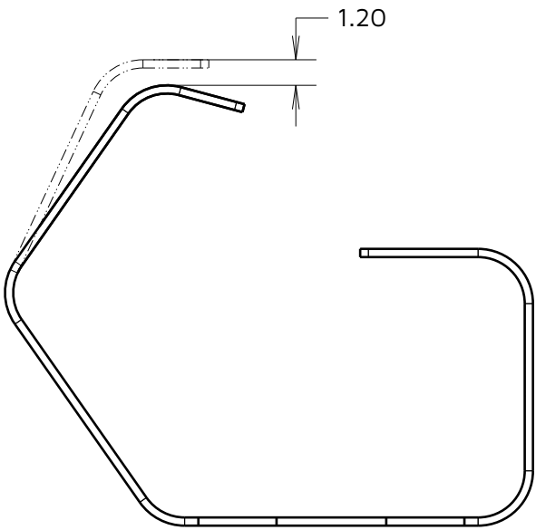
S1991-46R DEFLECTION FROM ABOVE
