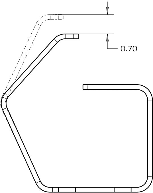
S1931-46R DEFLECTION FROM ABOVE
