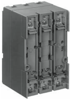
AQB-A101 Breaker with Single Front Connected Base
