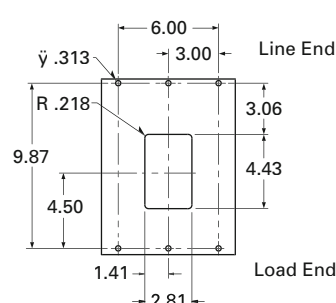
Minimum Front Panel Cutout
