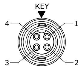
FACE VIEW P/N: CARA63804PXXX90
