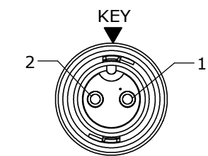
FACE VIEW P/N: CARA63802PXXX90
