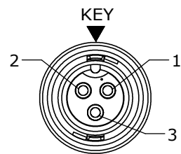
FACE VIEW P/N: CARA63803PXXX90
