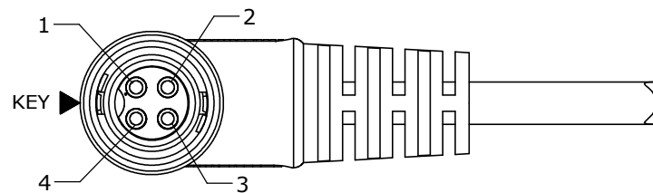
END "A" FACE VIEW SHOWN CARA63804PXXX90
