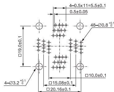
IC51-0484-806 (48 Pins)
