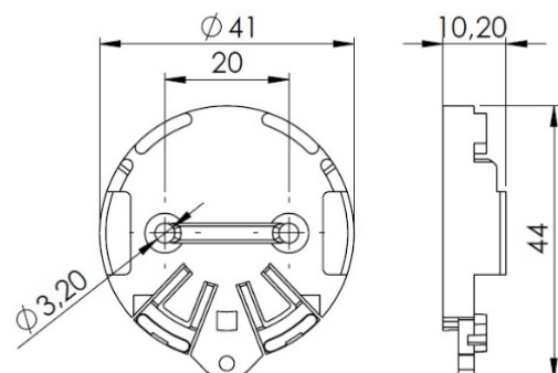
COIN HOLDER
