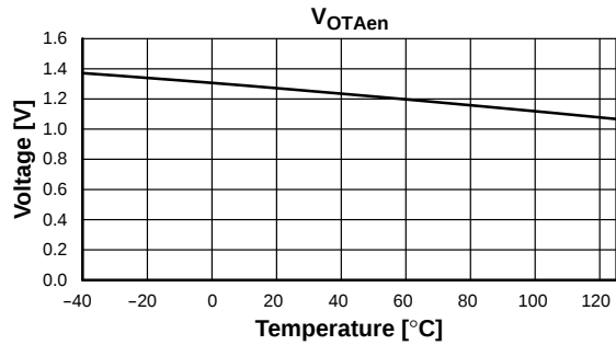
Figure 29. V OTAEen vs. Temperature
