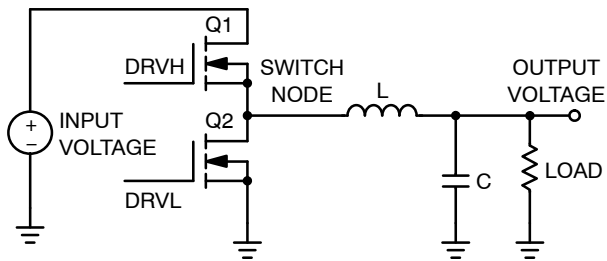
Figure 16. Buck Topology
