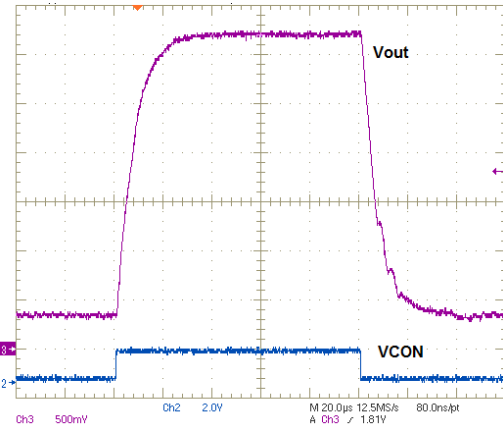
Figure 28. Transient, V_{OUT} vs. V_{CON} , R_L = 10\text{ }\Omega , V_{OUT} = 0.4\text{ V to } 3.6\text{ V} , PV_{IN} = 3.9\text{ V} w/ T_R = 7\text{ }\mu\text{s} , T_F = 10\text{ }\mu\text{s}
