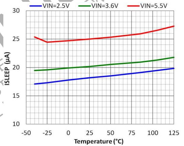
Figure 7. Sleep Mode Current vs Temperature ( EN = \text{High} , V_{CON} = 0\text{ V} , V_{OUT} = 0\text{ V} )
