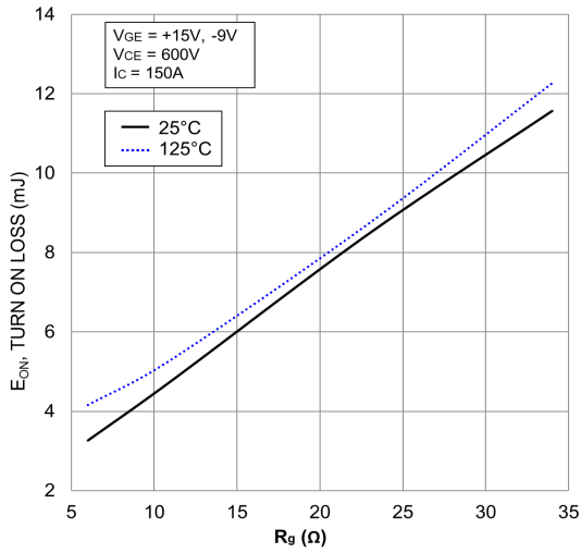
Figure 11. Typical Turn On Loss vs. R_g
