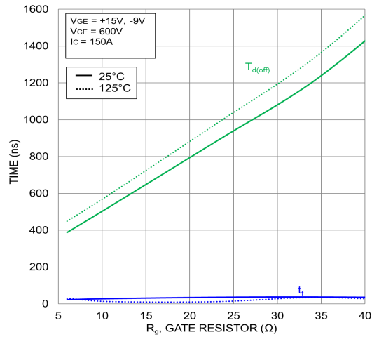
Figure 21. Typical Turn-Off Switching Time vs. R_G
