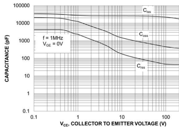
Figure 40. Capacitance Charge
