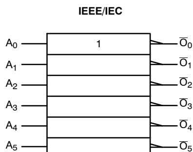
Figure 1. Logic Symbol
