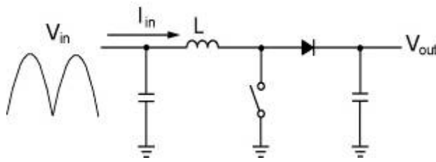
Figure 4. Boost Converter
