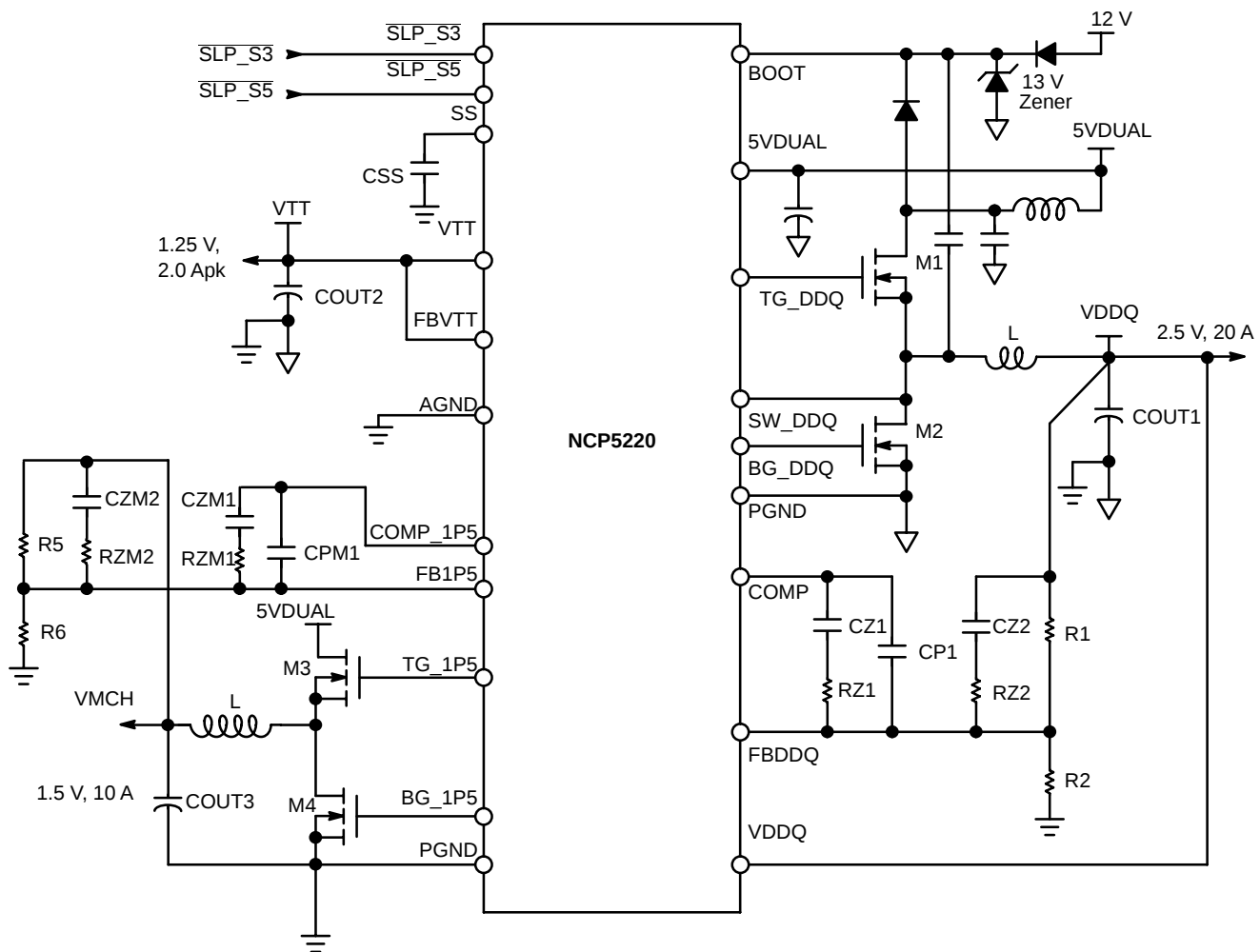
Figure 1. Application Diagram
