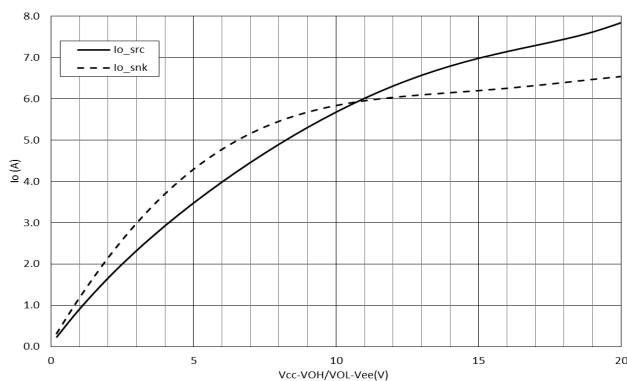
Figure 19. Output Current vs. Output Voltage Drop
