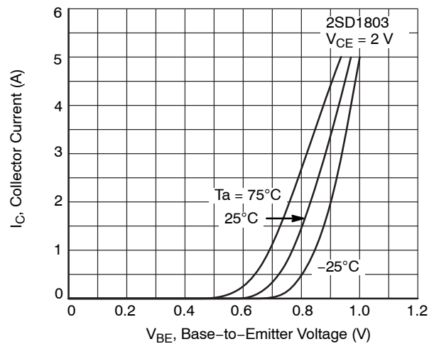
Figure 6. I_C - V_{BE}
