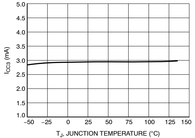
Figure 13. I CC3 vs. Temperature
