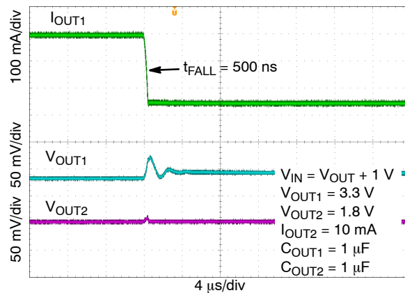
Figure 47. Load Transient Response – Falling Edge, I_{OUT} = 300 mA to 50 mA
