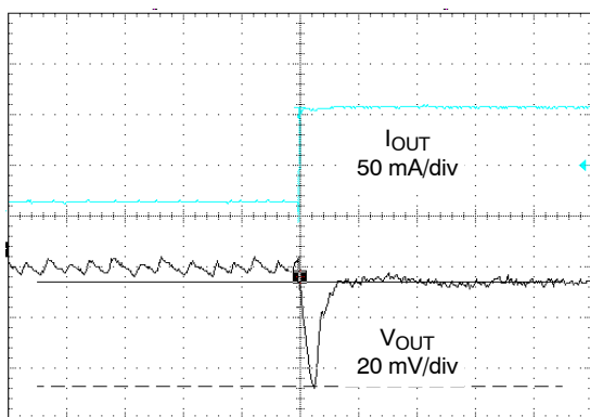
Figure 23. 10 mA to 100 mA Load Transient ( V_{IN} = 3.6 V, V_{OUT} = 1.2 V, T_A = 25^\circ\text{C} )
