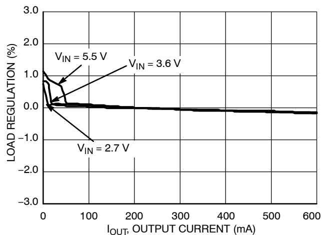
Figure 22. Load Regulation ( V_{OUT} = 1.2 V, T_A = 25^\circ\text{C} )
