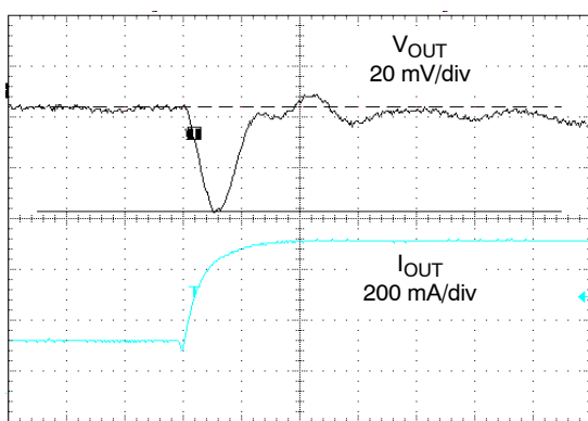
Figure 25. 200 mA to 600 mA Load Transient ( V_{IN} = 3.6 V, V_{OUT} = 1.2 V, T_A = 25^\circ\text{C} )
