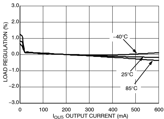
Figure 21. Load Regulation ( V_{IN} = 3.6 V, V_{OUT} = 1.2 V)
