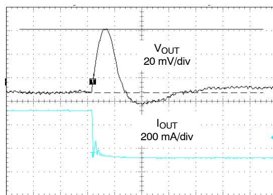
Figure 26. 600 mA to 200 mA Load Transient ( V_{IN} = 3.6 V, V_{OUT} = 1.2 V, T_A = 25^\circ\text{C} )
