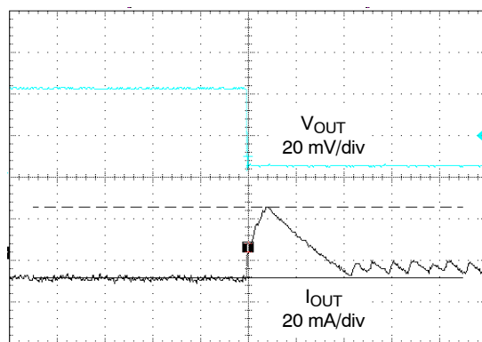
Figure 24. 100 mA to 10 mA Load Transient ( V_{IN} = 3.6 V, V_{OUT} = 1.2 V, T_A = 25^\circ\text{C} )
