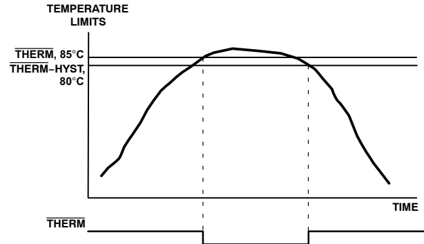
Figure 32. THERM Behavior
