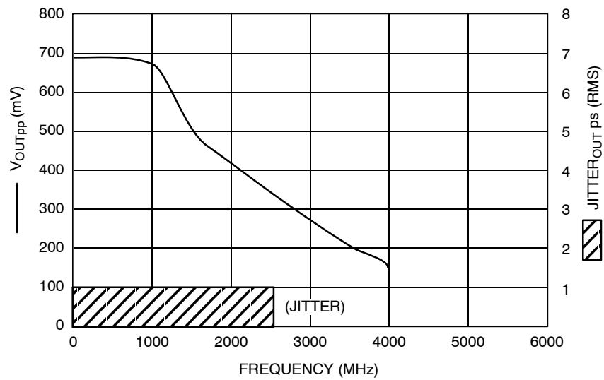
Figure 2. F_{max}/Jitter
