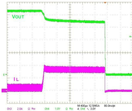
Figure 15. Overload Protection
