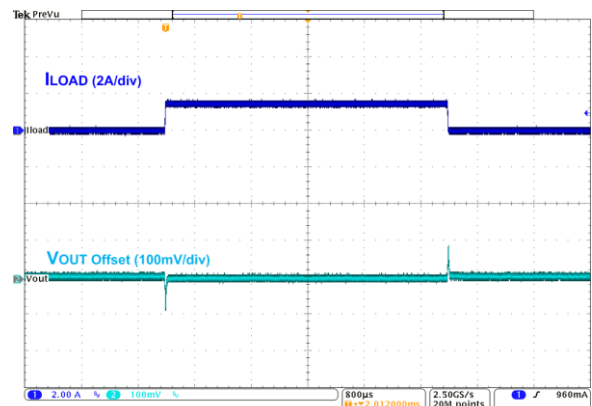
Figure 21. Load Transient, 0 mA \Rightarrow 1500 mA, 10 \mu s Edge, V_{IN} = 4.20\text{ V} , PWM Mode
