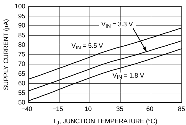
Figure 5. Quiescent Current vs. Temperature
