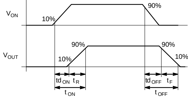
Figure 24. Timing Diagram
