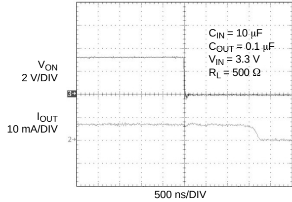
Figure 19. t_{dOFF} Response
