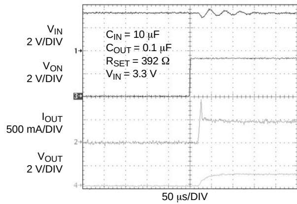
Figure 23. Current Limit Response Time (Output is Loaded by 2.2 \Omega , C_{OUT} = 10 \mu F )
