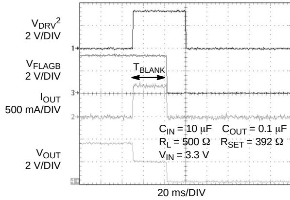
Figure 16. T_{BLANK} Response
