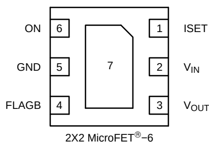
Figure 3. Pin Configuration
