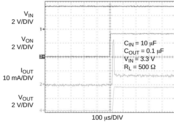
Figure 18. t_{dON} Response
