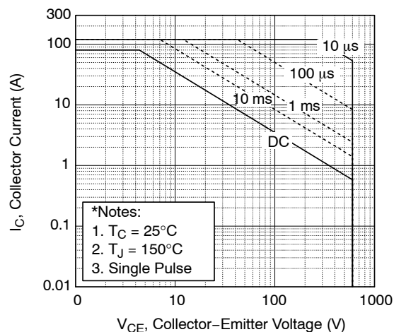
Figure 11. SOA Characteristics
