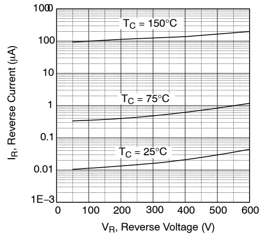
Figure 20. Reverse Current
