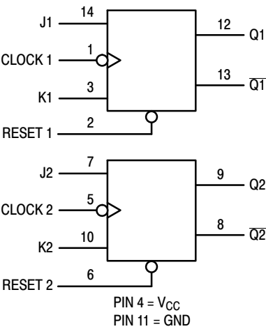
Figure 1. Logic Diagram
