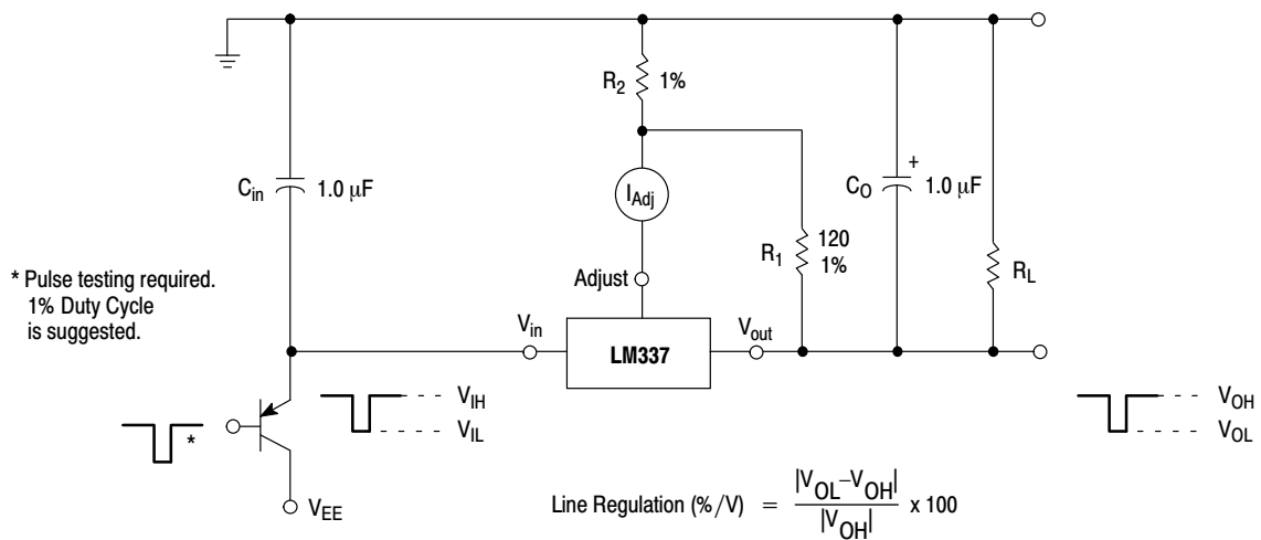
Figure 1. Line Regulation and \Delta I_{Adi} /Line Test Circuit
