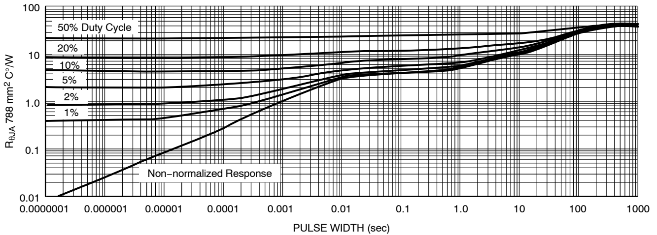
Figure 29. Duty Cycle for 1" Spreaders Boards, D 2 PAK 5-Lead
