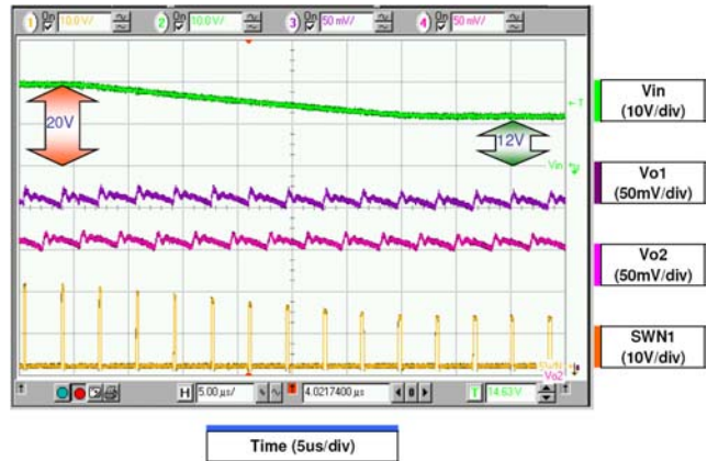
Figure 42. Line Transient Response ( V_{IN} = 20\text{ V} to 12\text{ V} , V_{O1} = 1.05\text{ V} , I_{O1} = 9\text{ A} , L_1 = 0.56\text{ }\mu\text{H} , C_{O1} = 470\text{ }\mu\text{F} \times 2 , V_{O2} = 1.05\text{ V} , I_{O2} = 9\text{ A} , L_2 = 0.56\text{ }\mu\text{H} , C_{O2} = 470\text{ }\mu\text{F} \times 2 , Dual-Channel Mode)
