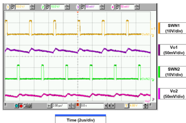
Figure 30. Output Voltage Ripple ( V_{IN} = 12\text{ V} , V_{O1} = 1.05\text{ V} , I_{O1} = 10\text{ A} , L1 = 0.56\text{ }\mu\text{H} , C_{O1} = 470\text{ }\mu\text{F} \times 2 , V_{O2} = 1.05\text{ V} , I_{O2} = 10\text{ A} , L2 = 0.56\text{ }\mu\text{H} , C_{O2} = 470\text{ }\mu\text{F} \times 2 , Dual-Channel Operation)
