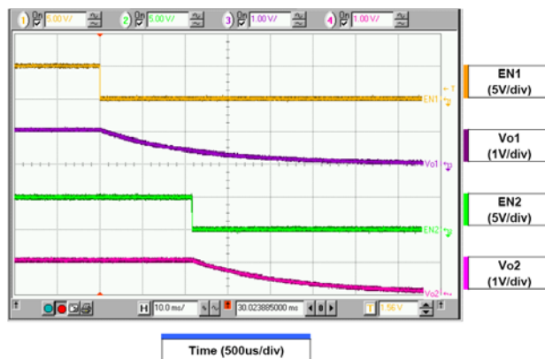
Figure 34. Powerdown and Soft-Stop ( V_{IN} = 12\text{ V} , V_{O1} = 1.05\text{ V} , I_{O1} = 0\text{ A} , V_{O2} = 1.05\text{ V} , I_{O2} = 0\text{ A} , Dual-Channel Operation)
