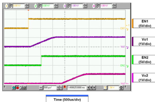
Figure 32. Powerup with EN2 Comes before CH1 Completes Soft-Start ( V_{IN} = 12\text{ V} , V_{O1} = 1.05\text{ V} , I_{O1} = 0\text{ A} , V_{O1} = 1.05\text{ V} , I_{O2} = 0\text{ A} , Dual-Channel Operation)
