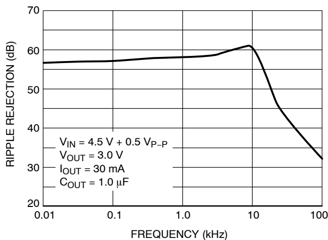
Figure 7. Ripple Rejection/Frequency
