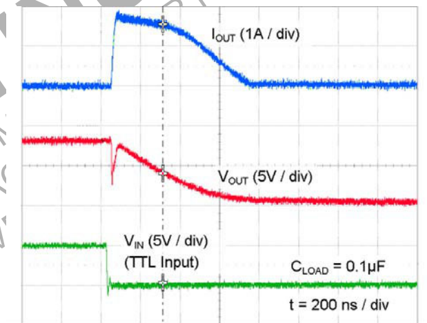
Figure 25. Quasi-Static Sink Current with V_{DD} = 8\text{ V}
