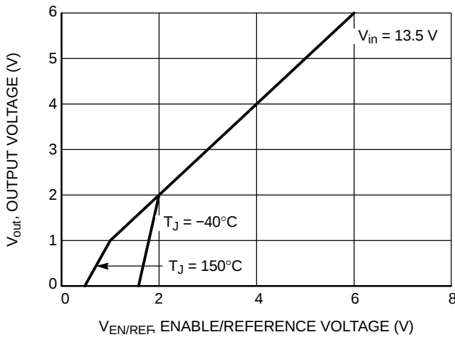
Figure 3. Output Voltage V_{out} vs. Reference Voltage V_{EN/REF}
