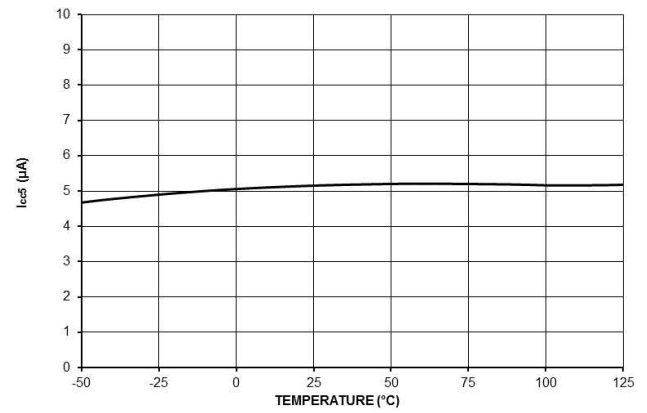
Figure 35. Internal Current Consumption in Off Mode I CC5
