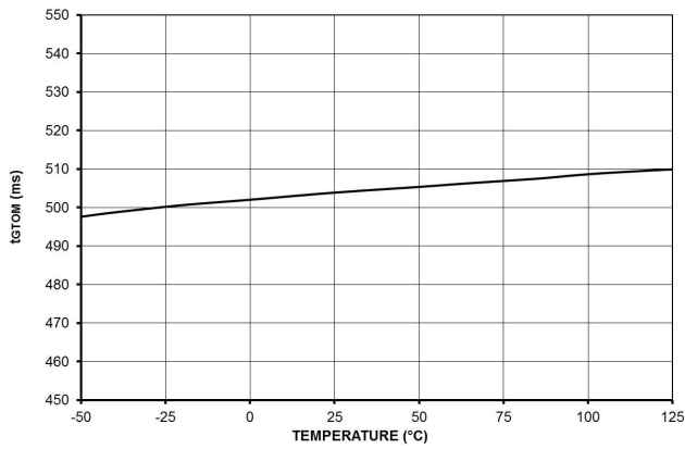
Figure 34. Go To Off Mode Timer Duration t GTOM
