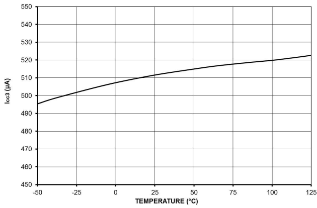
Figure 32. Internal Current Consumption in Skip Mode I CC3
