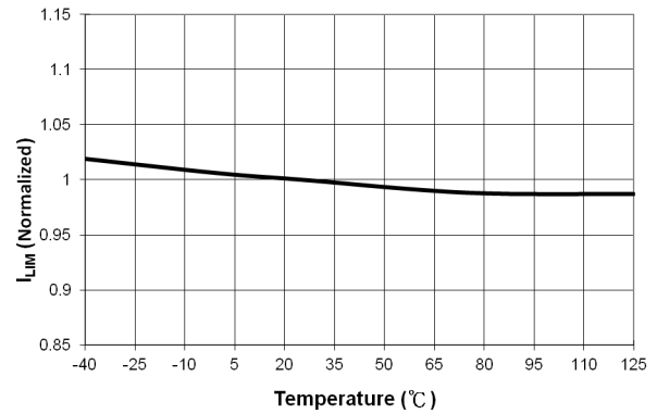
Figure 16. FSL538A I_{LIM} (Normalized to 25°C) vs. Temperature
