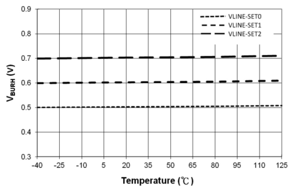
Figure 22. V_{BURH} vs. Temperature
