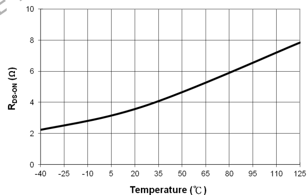
Figure 26. FSL538H/A R_{DS(ON)} vs. Temperature
