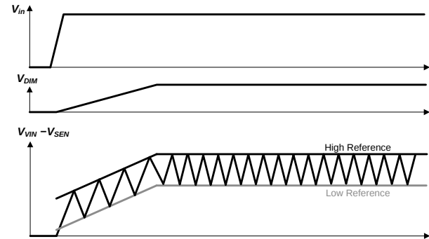
Figure 18. Soft Start with DIM pin Capacitor
