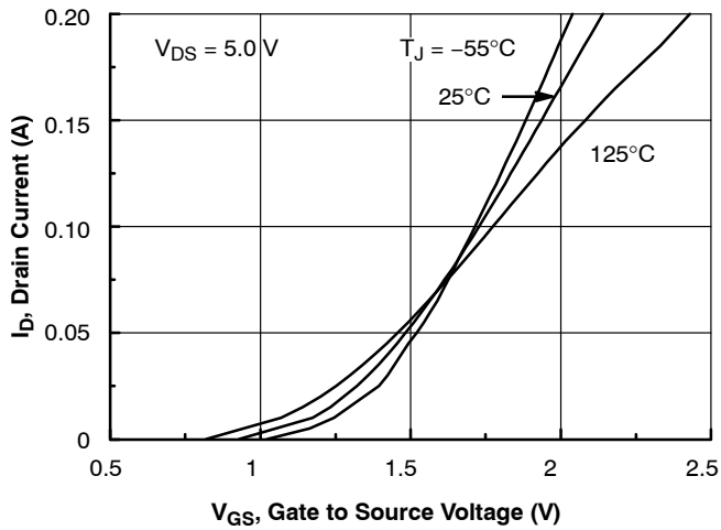
Figure 6. Transfer Characteristics
