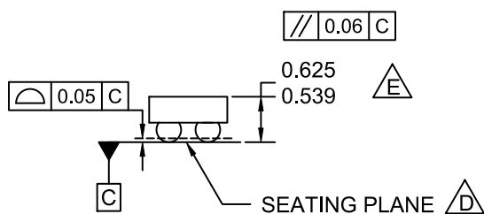
SIDE VIEWS
