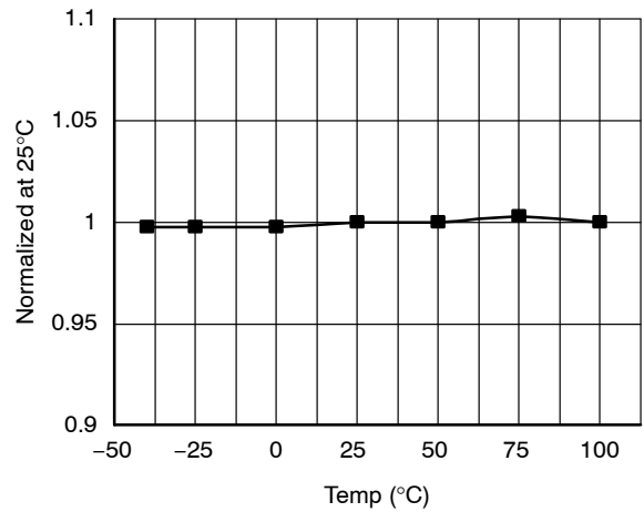
Figure 15. OCP Voltage vs. Temperature
