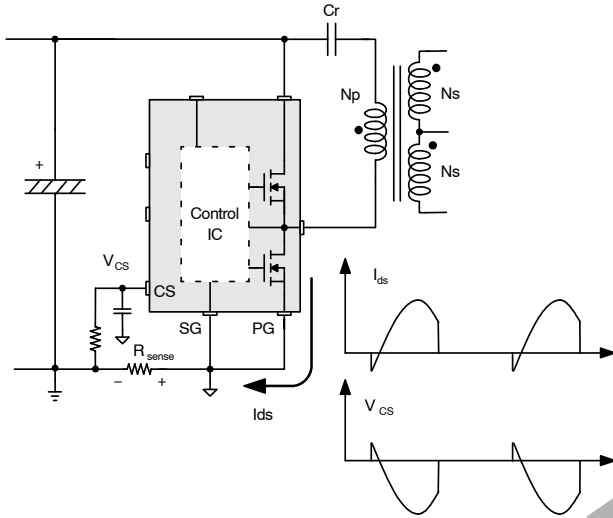
Figure 24. Half-Wave Sensing
