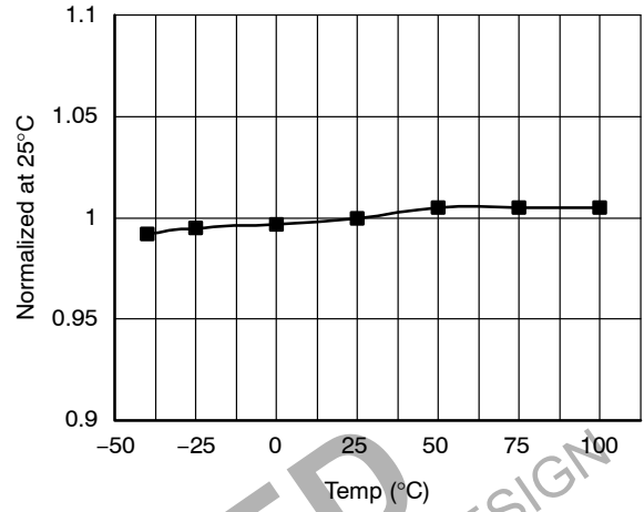
Figure 11. OLP Protection Voltage vs. Temperature
