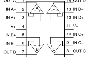
TSSOP-14
