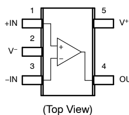
SC70-5/TSOP-5
