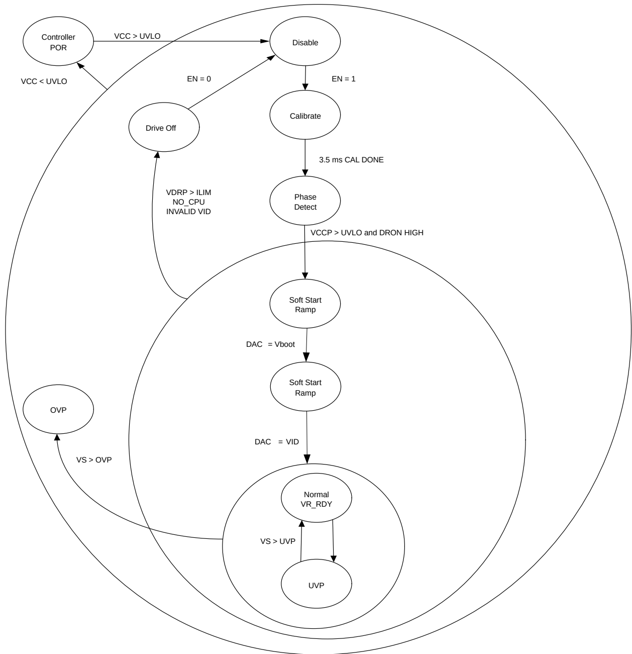
Figure 6. State Diagram
