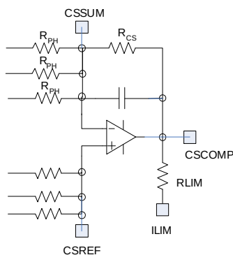
Figure 21. I_{lim} Resistor
